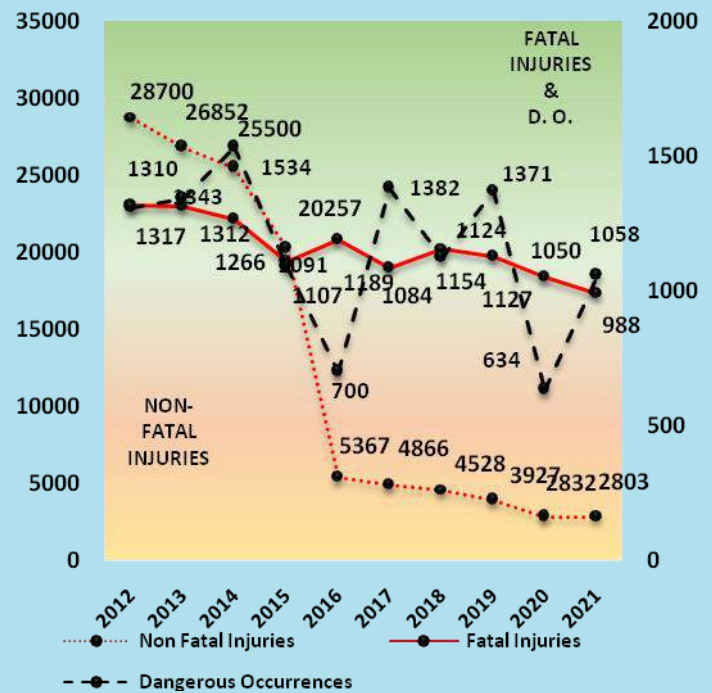
Graph 6: Fatal Injuries, Non-fatal Injuries and Dangerous Occurrences in Registered factories in India (2012-2021)
