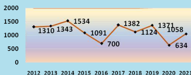
Graph 3: Dangerous Occurrences in Registered factories in India (2012-2021)
